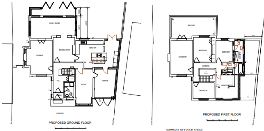
Figure 5: Proposed Floorplans
