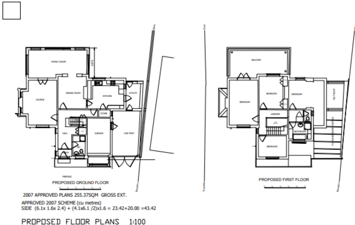
Figure 5: Proposed Floorplans
